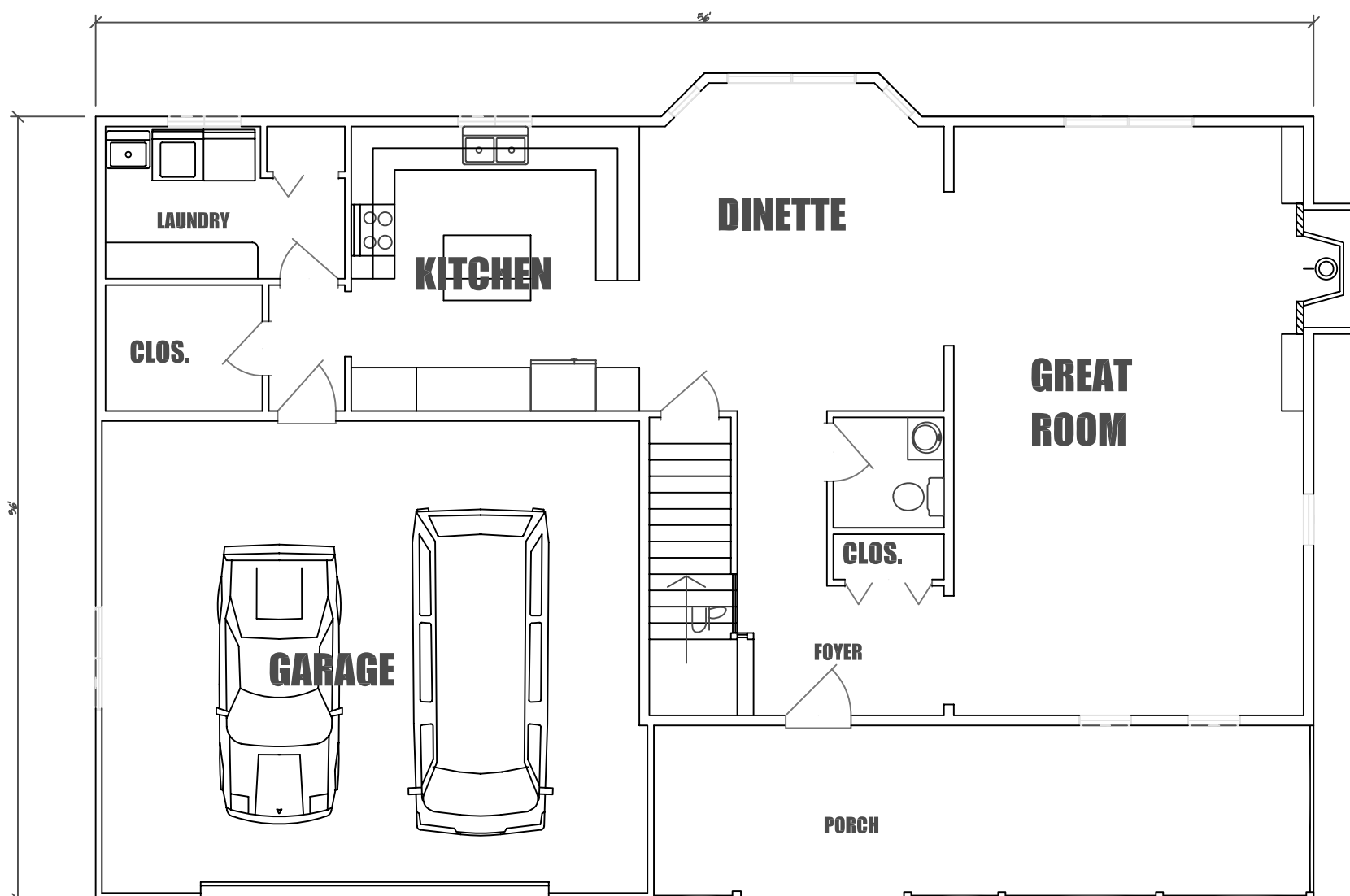
Main Level Plan
